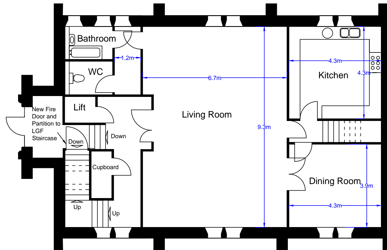
8DT14: 8 Derby Terrace Ground Floor as Proposed Page 1 of 1, Scale 1:100 at A3
